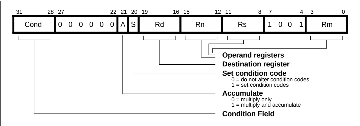
Figure 4-12: Multiply instructions
