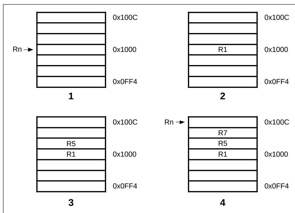
Figure 4-19: Post-increment addressing
